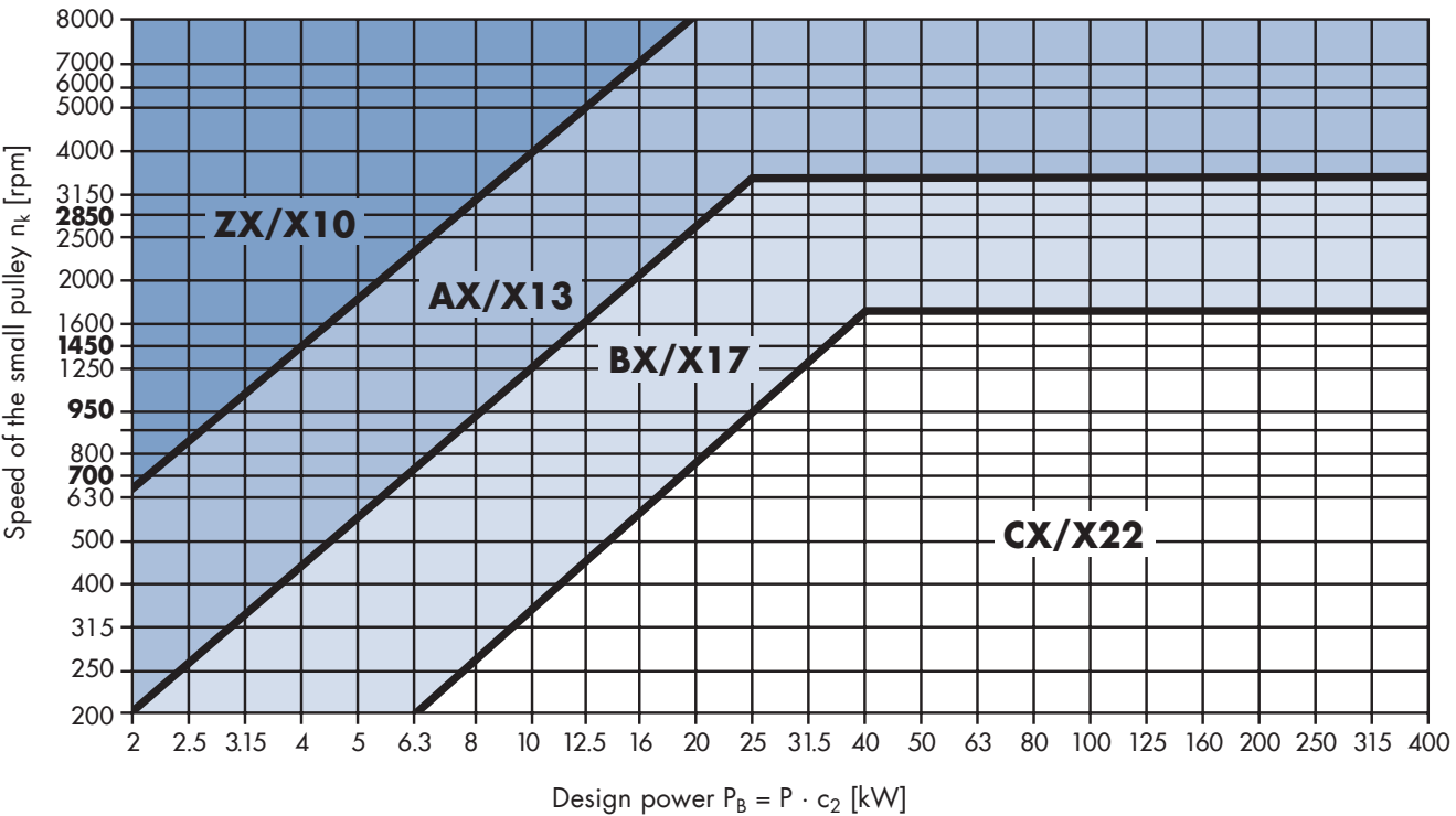
Diagram 5: optibelt SUPER TX M=S V-belts
